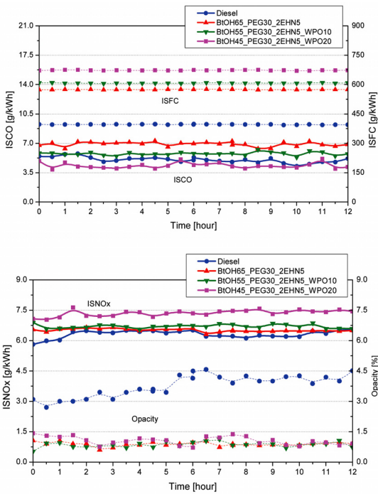
Fig. 10 Duration test - CO, NOx, Soot emissions and ISFC as a function of time with various test fuels at generator output 3.3 kW e
